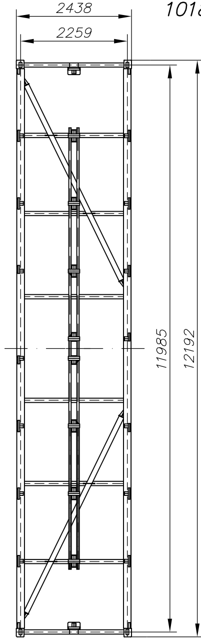
VIEW X
