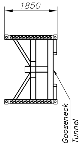
VIEW X
