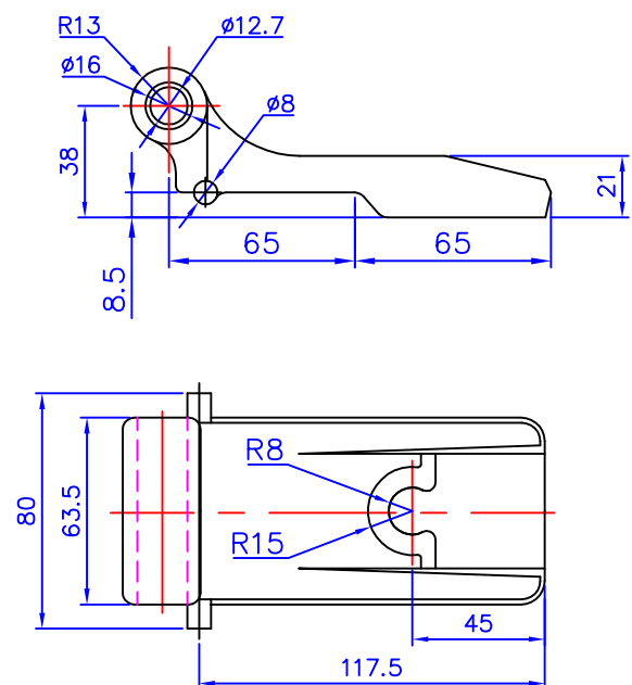
PMI-D24-04 Maersk Type
