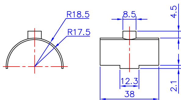
PMI-D23-14 Upper Short Split Bush
