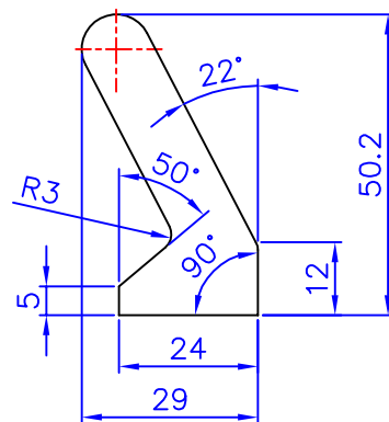
PMI-D30-03 Ø12X140 For Top and Bottom Side Rail
