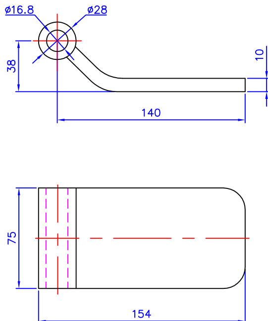
PMI-D24-03 Welded Type
