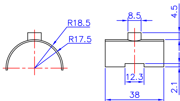
PMI-D23-15 Lower Short Split Bush
