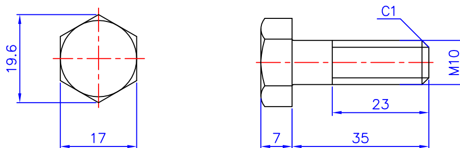
PMI-D27-02 Door Screw M10X35
