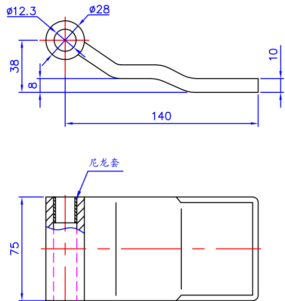
PMI-D24-02 Welded Type
