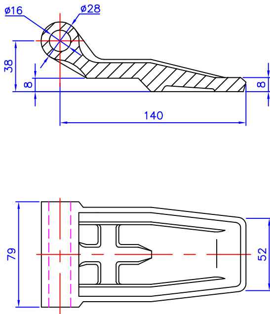
PMI-D24-01 Forged Type
