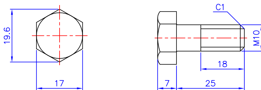
PMI-D27-01 Door Screw M10X25
