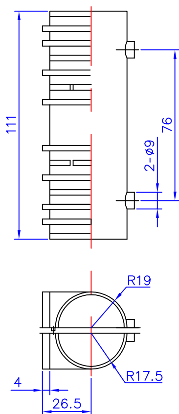
PMI-D23-16 Split Large Bush
