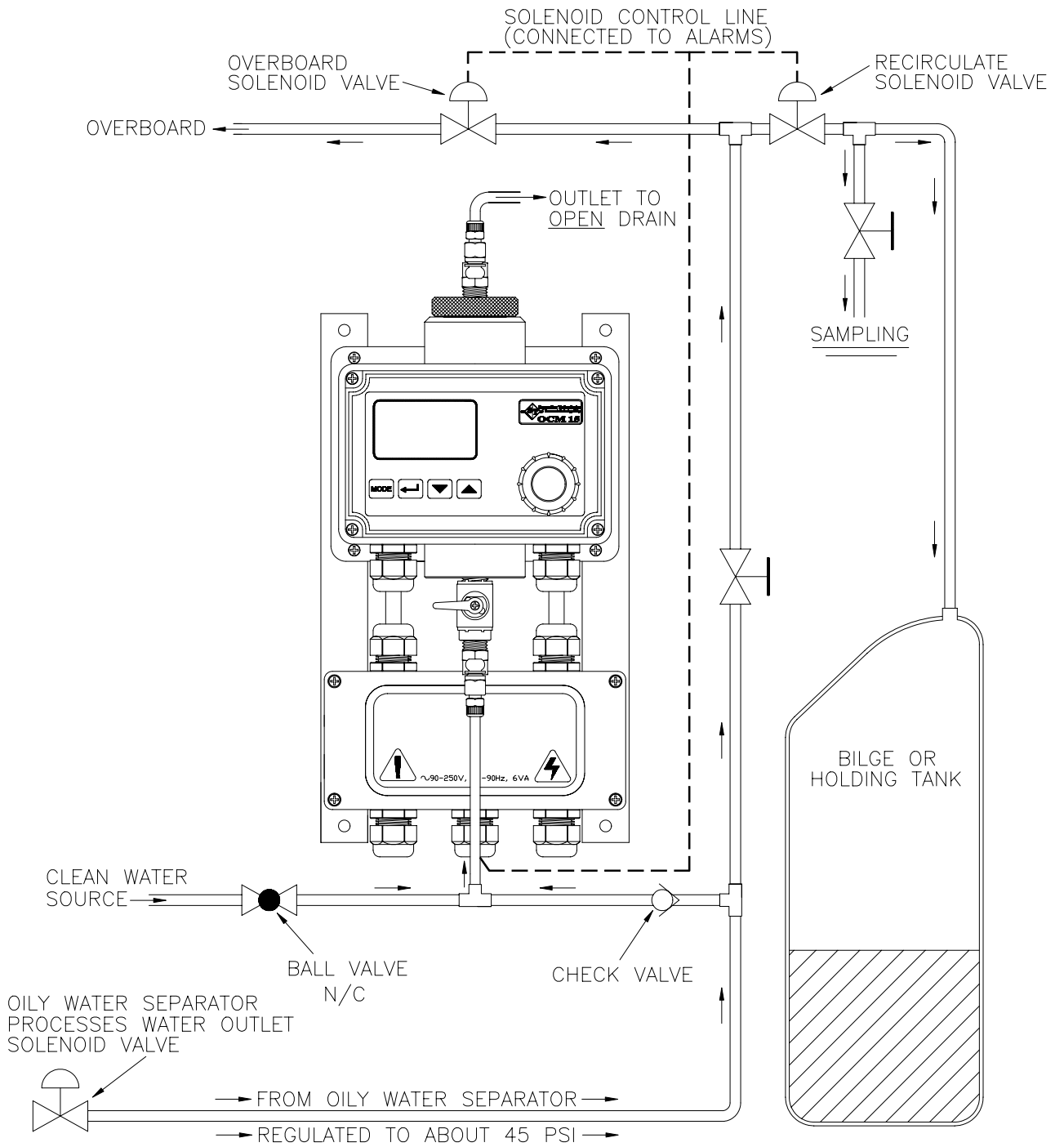
Figure 2: Recommended Plumbing for the instrument.
